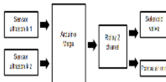
Gambar 3. Blok Diagram
